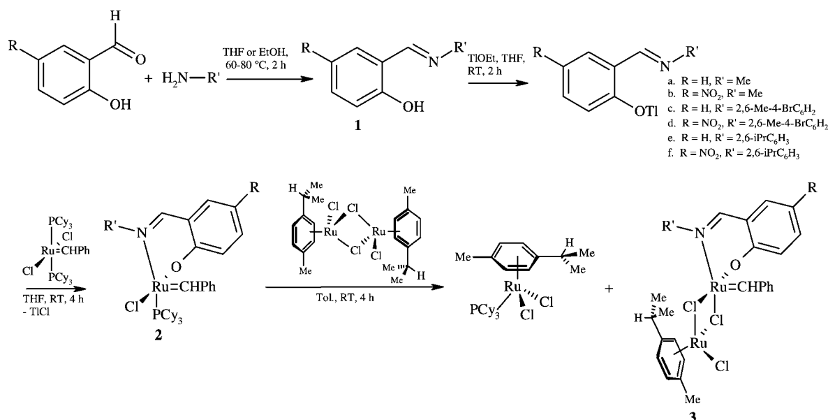
Scheme 1. Synthesis route of the different catalytic systems.
